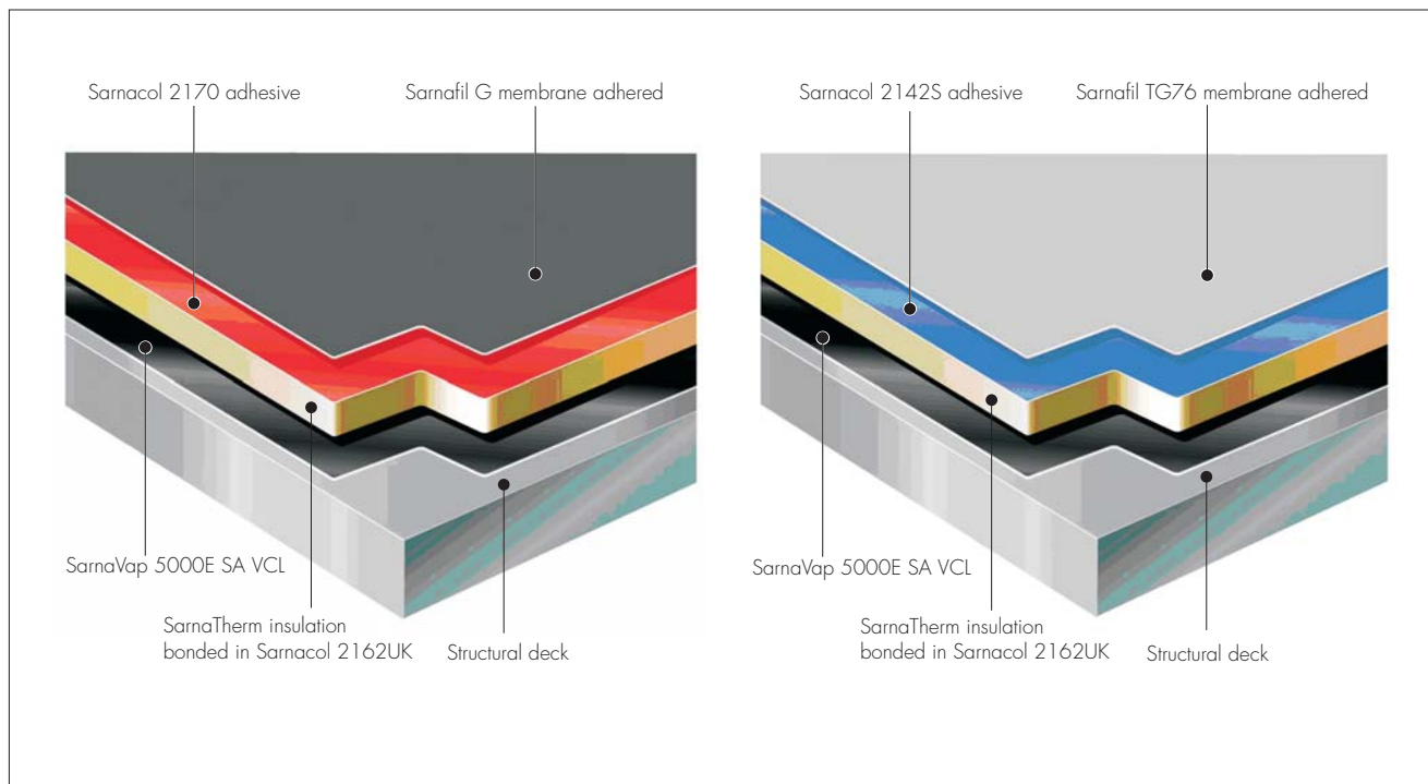
Figure 1 Typical installations
